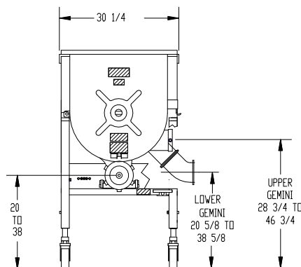
Model 120 Bulker
